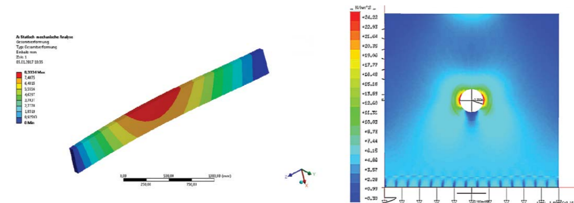
Deformation of the glass beam with a height of 300mm under full load conditions (ULS) and in induced imperfection of 1/400 = 6,5 mm
